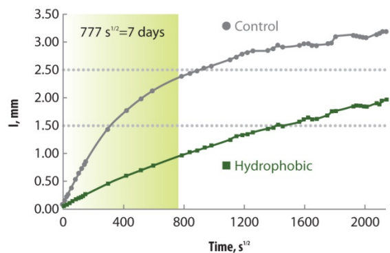
Determination of Capillary Absorption ASTM C1585
